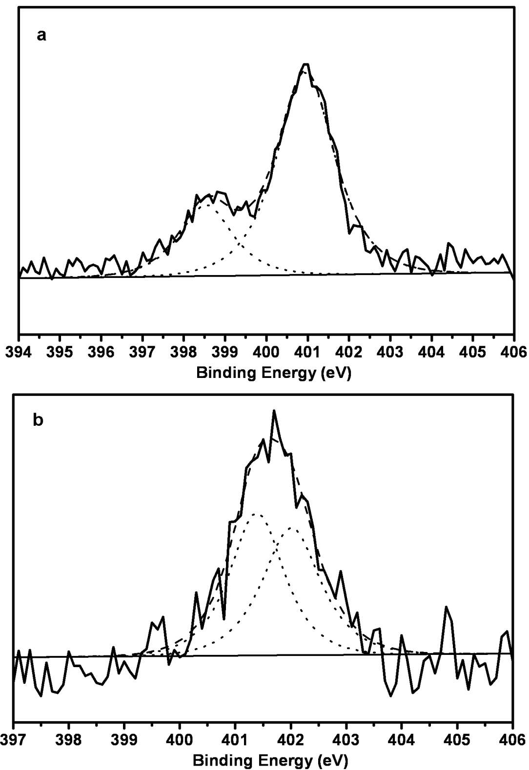
Figure S13. N 1s XPS spectra of (a). BuV, (b). CT cocrystals (solid line: experimental energy curves, dot line: assigning peak energy curves).
