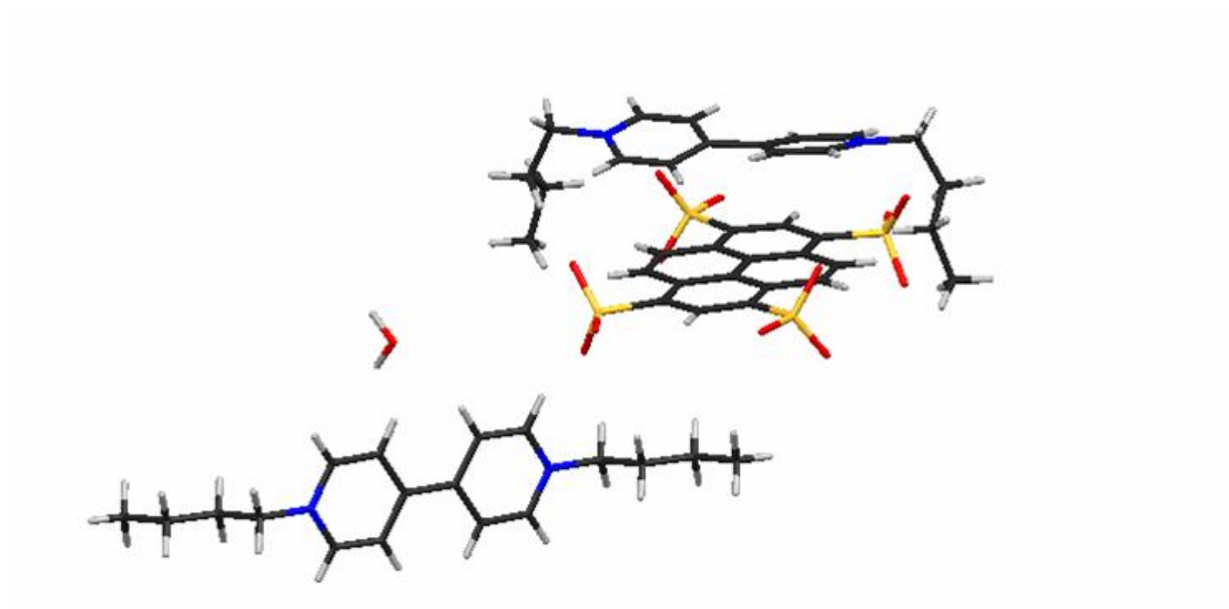
Figure S8. Crystal structure of the CT cocrystal by stick mode (yellow: S, red: O, blue: N, dark gray: C, light gray: H).
